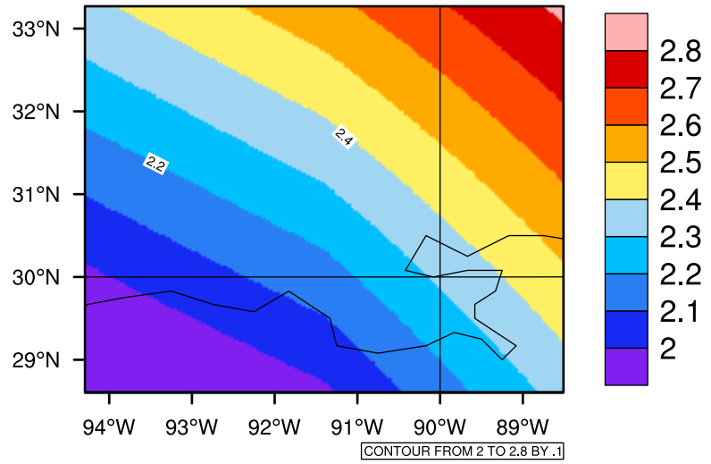
Yearly pr (mm/day) In 2090-2099 GFDL-ESM2M RCP45 - Louisiana
