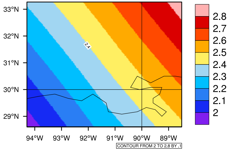
Yearly pr (mm/day) In 2030-2039 GFDL-ESM2M RCP85 - Louisiana
