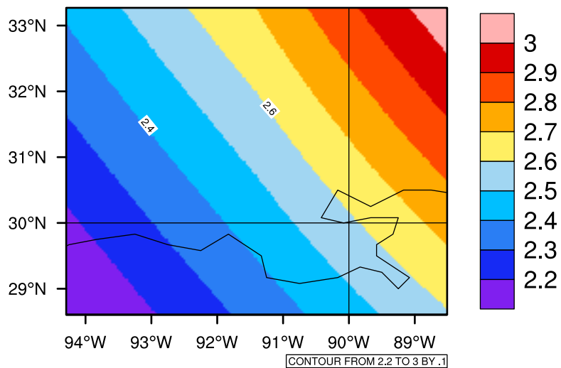
Yearly pr (mm/day) In 2040-2049 GFDL-ESM2M RCP85 - Louisiana
