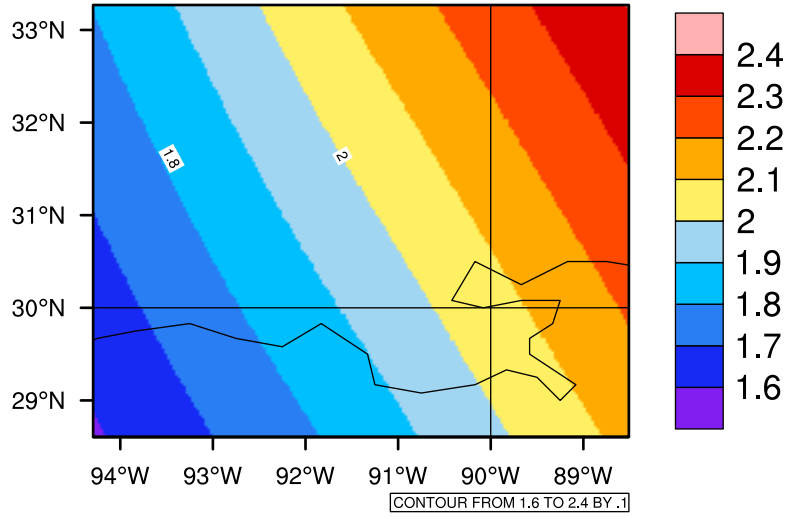
Yearly pr (mm/day) In 2070-2079 GFDL-ESM2M RCP85 - Louisiana
