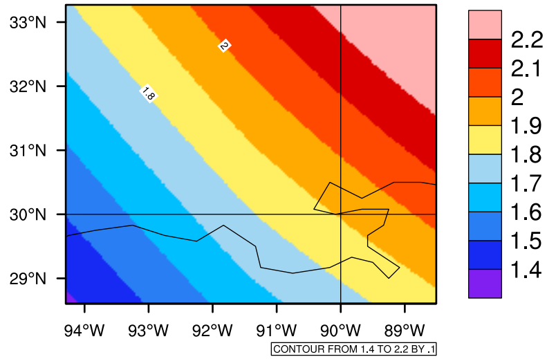
Yearly pr (mm/day) In 2090-2099 GFDL-ESM2M RCP85 - Louisiana
