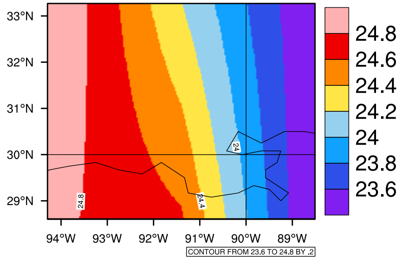
Yearly tasmax(c) In 2050-2059 GFDL-ESM2M RCP45 - Louisiana
