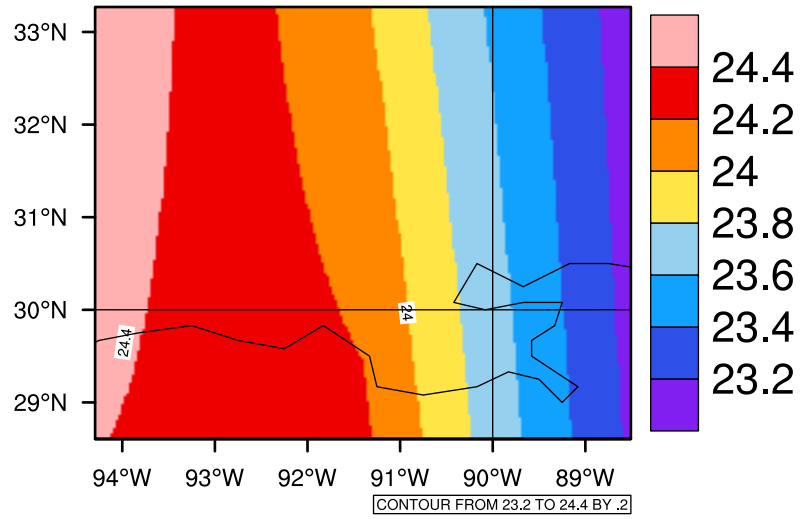
Yearly tasmax(c) In 2030-2039 GFDL-ESM2M RCP85 - Louisiana
