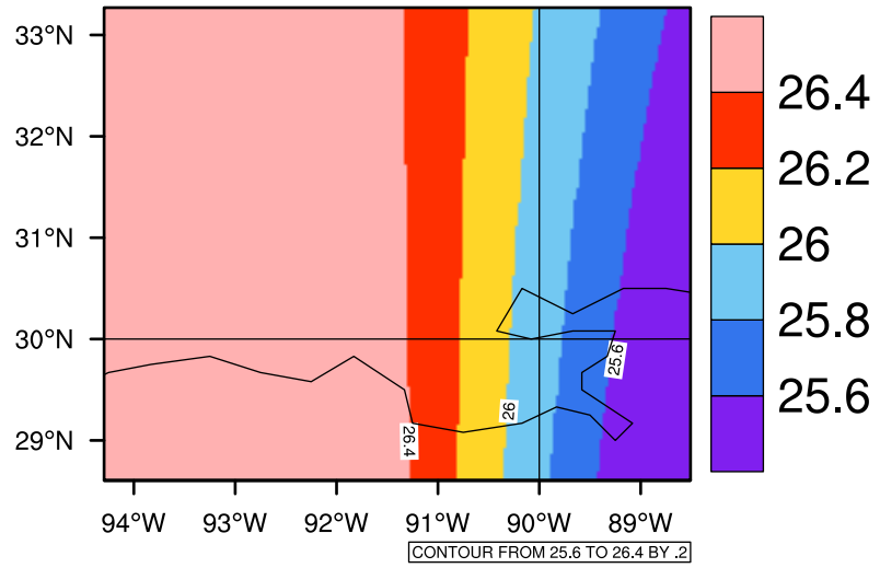
Yearly tasmax(c) In 2080-2089 GFDL-ESM2M RCP85 - Louisiana
