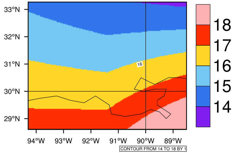
Yearly tasmin(c) In 2020-2029 GFDL-ESM2M RCP45 - Louisiana
