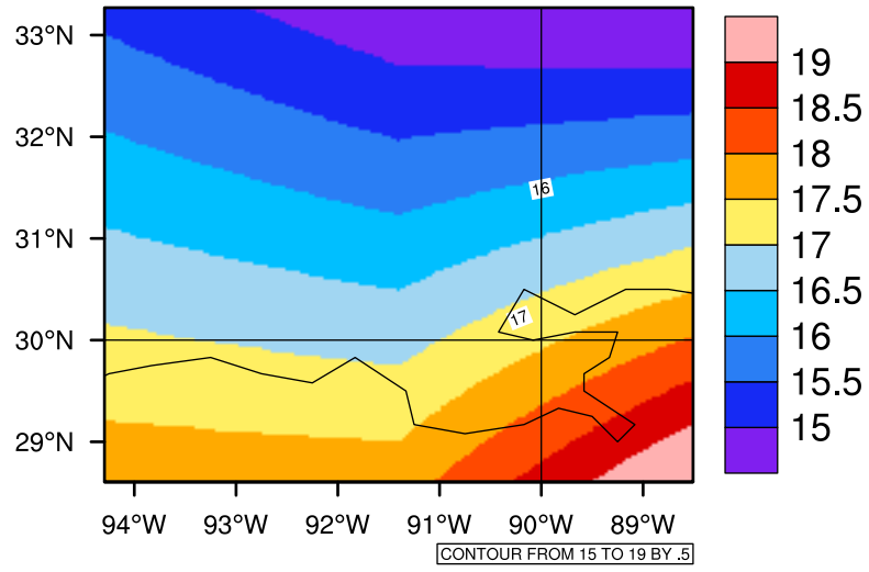
Yearly tasmin(c) In 2040-2049 GFDL-ESM2M RCP45 - Louisiana
