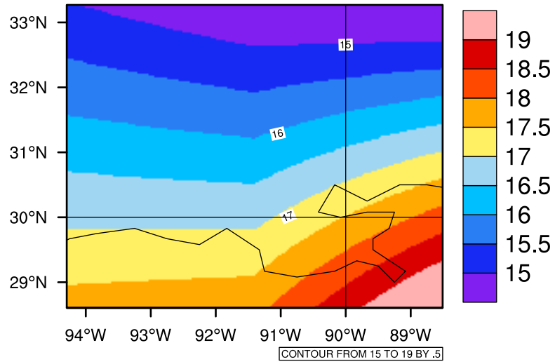
Yearly tasmin(c) In 2060-2069 GFDL-ESM2M RCP45 - Louisiana
