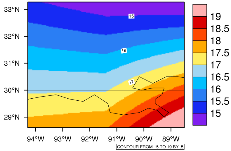
Yearly tasmin(c) In 2070-2079 GFDL-ESM2M RCP45 - Louisiana
