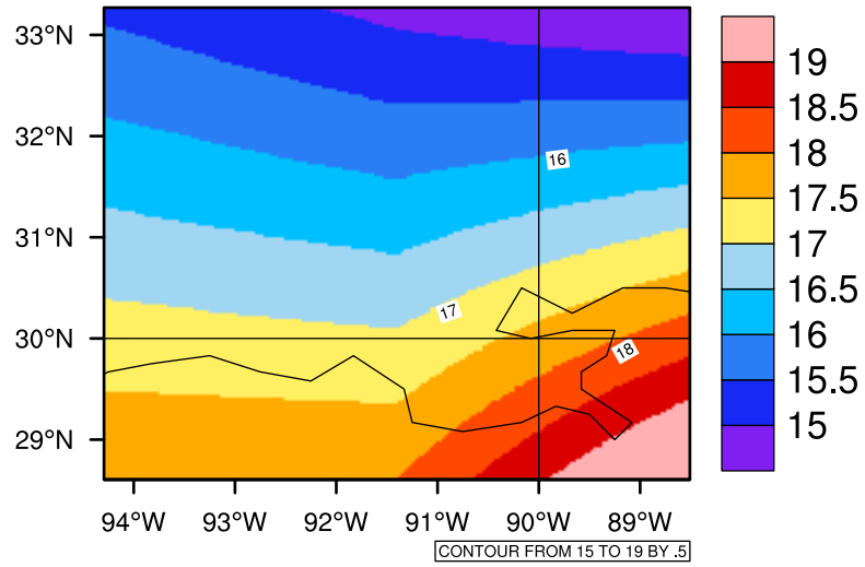
Yearly tasmin(c) In 2080-2089 GFDL-ESM2M RCP45 - Louisiana
