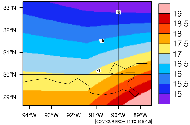
Yearly tasmin(c) In 2090-2099 GFDL-ESM2M RCP45 - Louisiana
