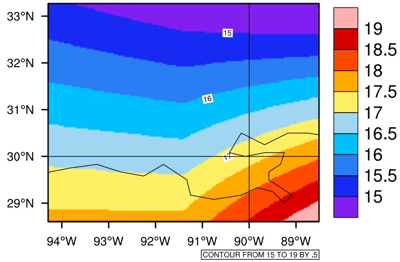
Yearly tasmin(c) In 2030-2039 GFDL-ESM2M RCP85 - Louisiana
