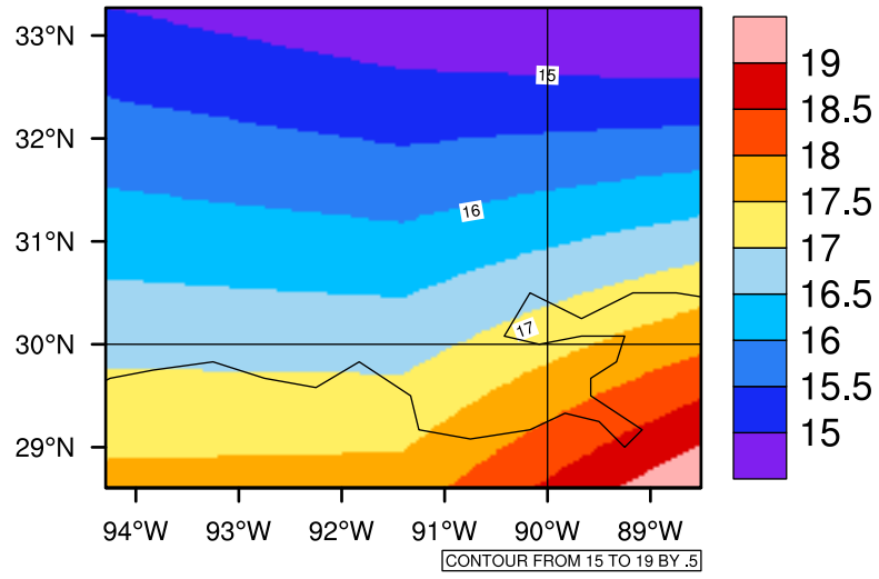
Yearly tasmin(c) In 2040-2049 GFDL-ESM2M RCP85 - Louisiana
