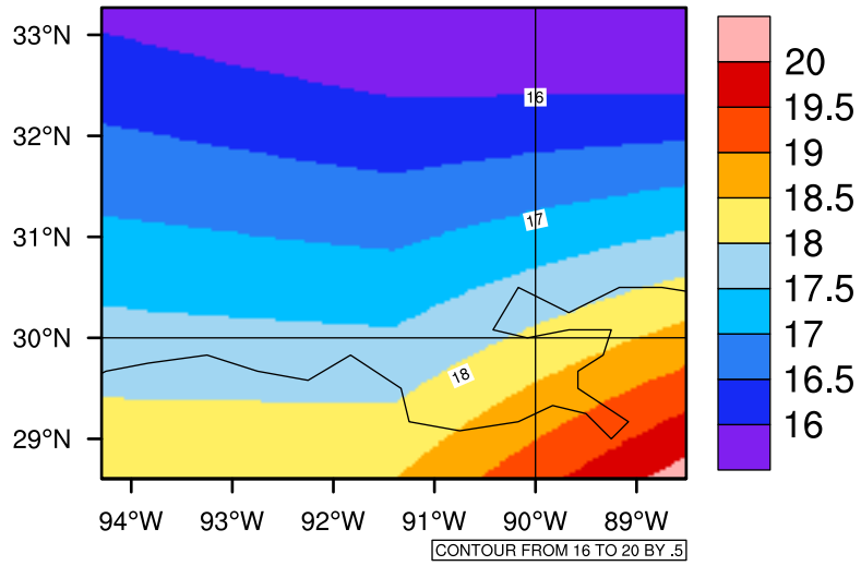
Yearly tasmin(c) In 2050-2059 GFDL-ESM2M RCP85 - Louisiana
