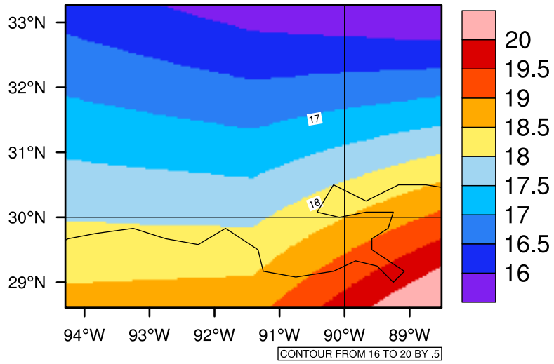
Yearly tasmin(c) In 2060-2069 GFDL-ESM2M RCP85 - Louisiana
