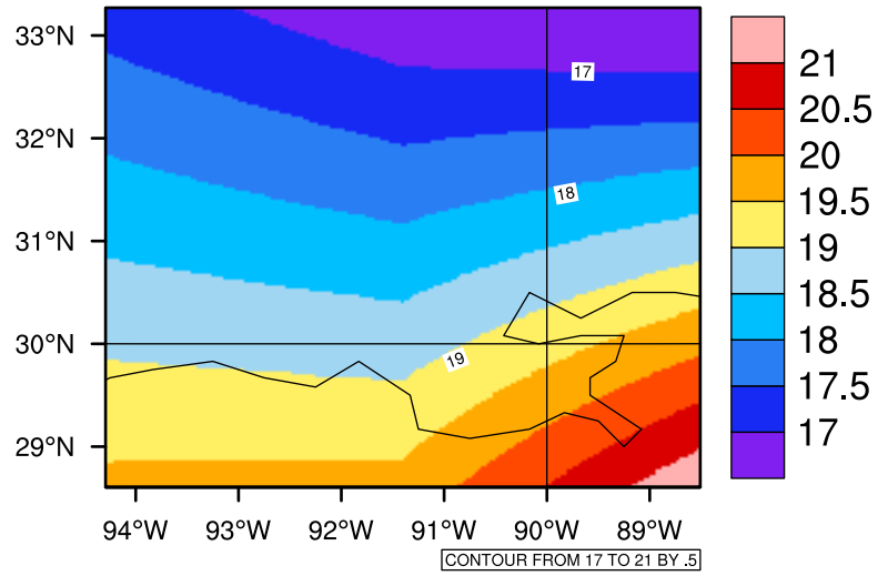
Yearly tasmin(c) In 2080-2089 GFDL-ESM2M RCP85 - Louisiana
