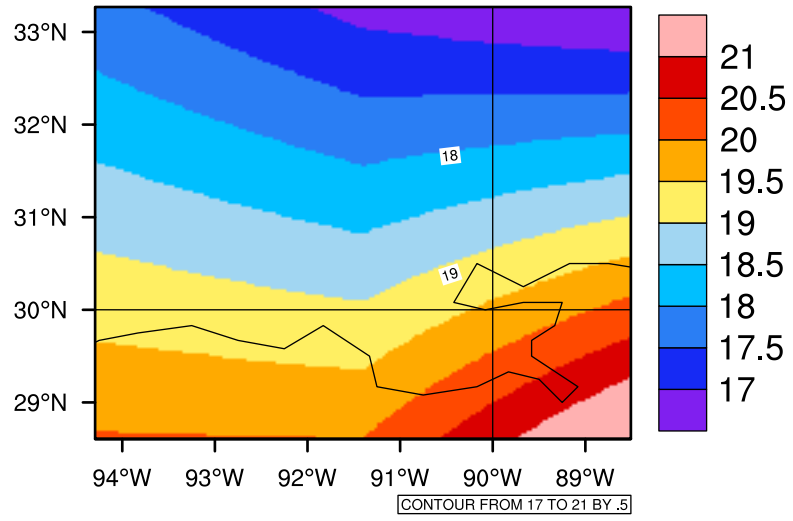
Yearly tasmin(c) In 2090-2099 GFDL-ESM2M RCP85 - Louisiana
