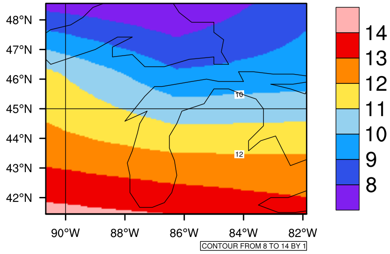
Yearly tasmax(c) In 2050-2059 GFDL-ESM2M RCP45 - Michigan
