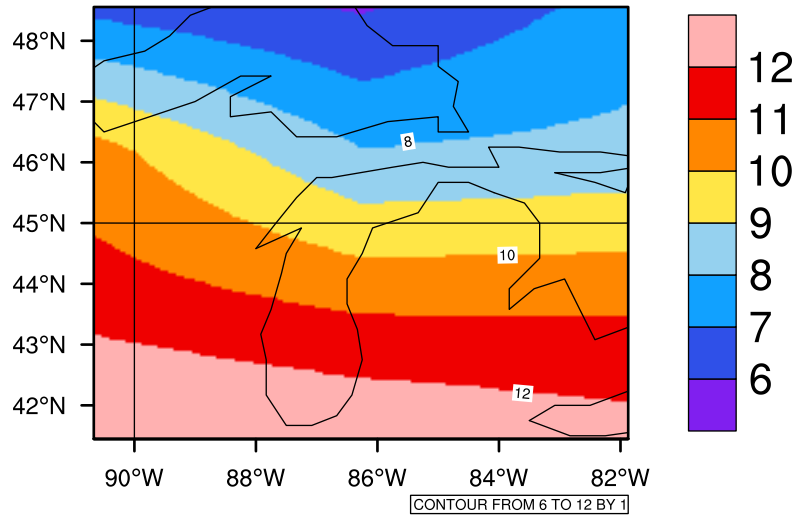
Yearly tasmax(c) In 2020-2029 GFDL-ESM2M RCP85 - Michigan
