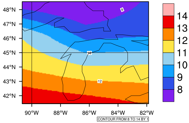
Yearly tasmax(c) In 2040-2049 GFDL-ESM2M RCP85 - Michigan
