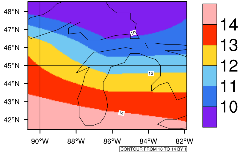
Yearly tasmax(c) In 2050-2059 GFDL-ESM2M RCP85 - Michigan
