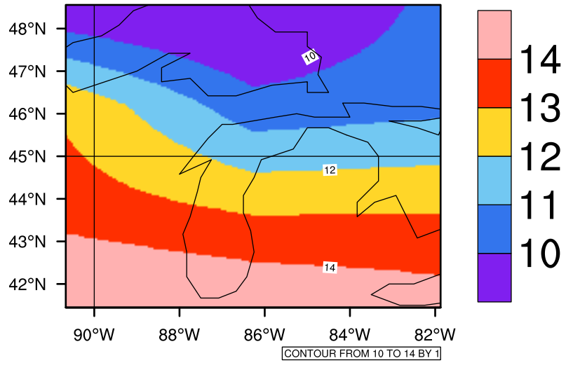
Yearly tasmax(c) In 2060-2069 GFDL-ESM2M RCP85 - Michigan
