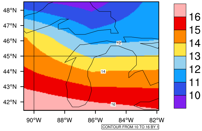
Yearly tasmax(c) In 2090-2099 GFDL-ESM2M RCP85 - Michigan
