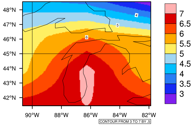
Yearly tasmin(c) In 2020-2029 GFDL-ESM2M RCP45 - Michigan
