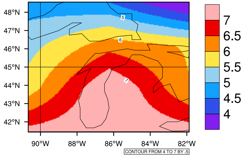
Yearly tasmin(c) In 2040-2049 GFDL-ESM2M RCP45 - Michigan
