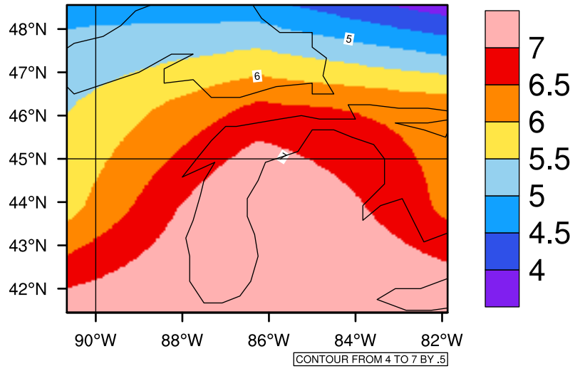
Yearly tasmin(c) In 2050-2059 GFDL-ESM2M RCP45 - Michigan
