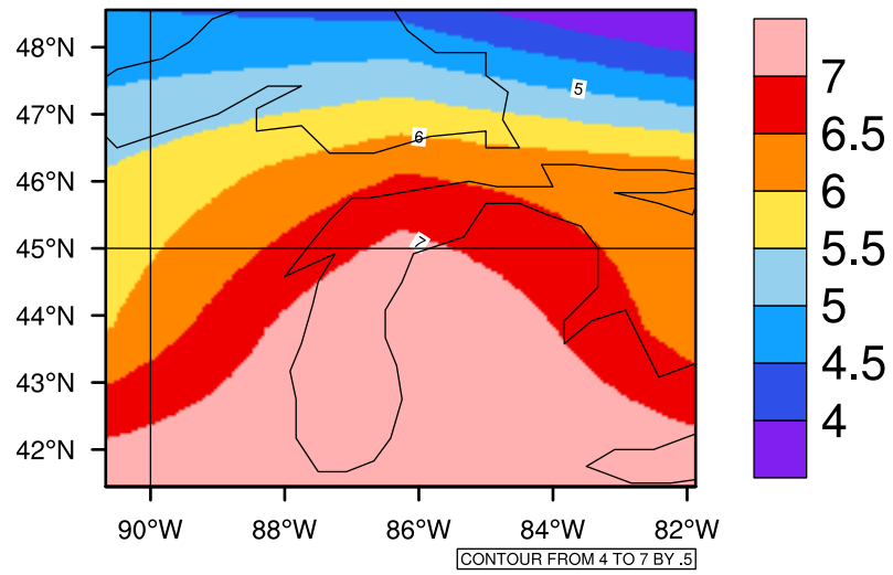
Yearly tasmin(c) In 2070-2079 GFDL-ESM2M RCP45 - Michigan
