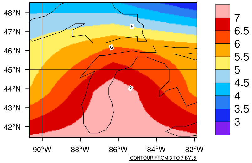
Yearly tasmin(c) In 2040-2049 GFDL-ESM2M RCP85 - Michigan
