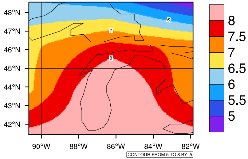
Yearly tasmin(c) In 2050-2059 GFDL-ESM2M RCP85 - Michigan
