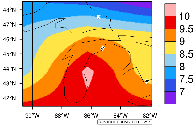
Yearly tasmin(c) In 2090-2099 GFDL-ESM2M RCP85 - Michigan
