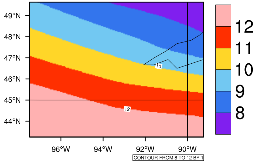
Yearly tasmax(c) In 2020-2029 GFDL-ESM2M RCP45 - Minnesota
