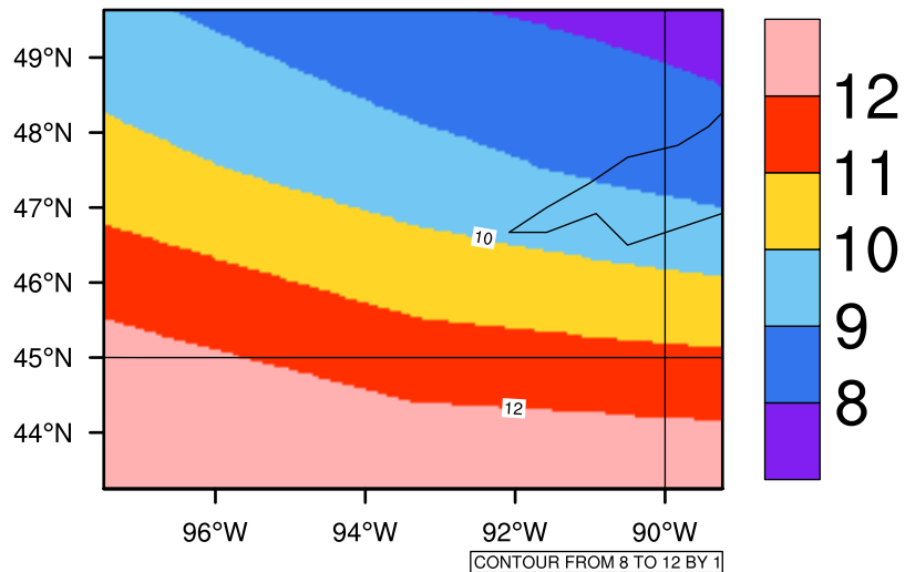
Yearly tasmax(c) In 2050-2059 GFDL-ESM2M RCP45 - Minnesota
