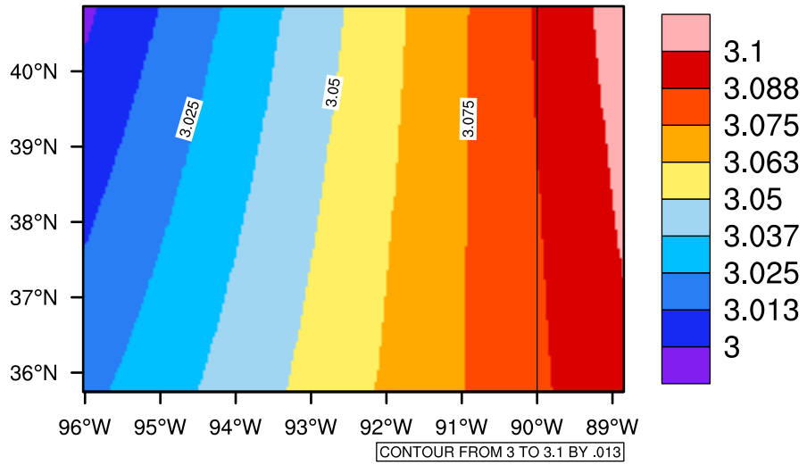
Yearly pr (mm/day) In 2020-2029 GFDL-ESM2M RCP45 - Missouri
