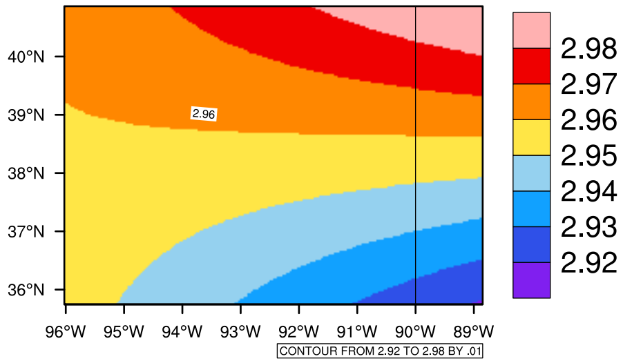
Yearly pr (mm/day) In 2030-2039 GFDL-ESM2M RCP45 - Missouri
