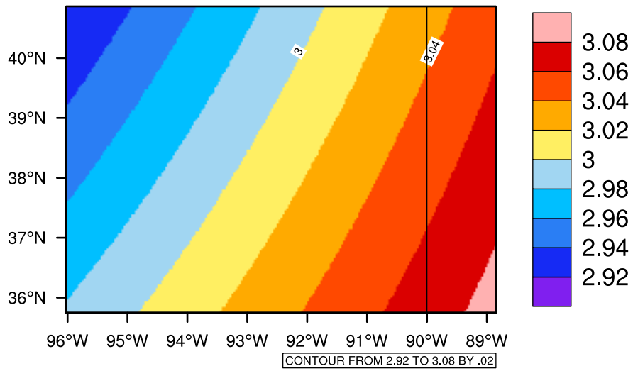
Yearly pr (mm/day) In 2040-2049 GFDL-ESM2M RCP45 - Missouri
