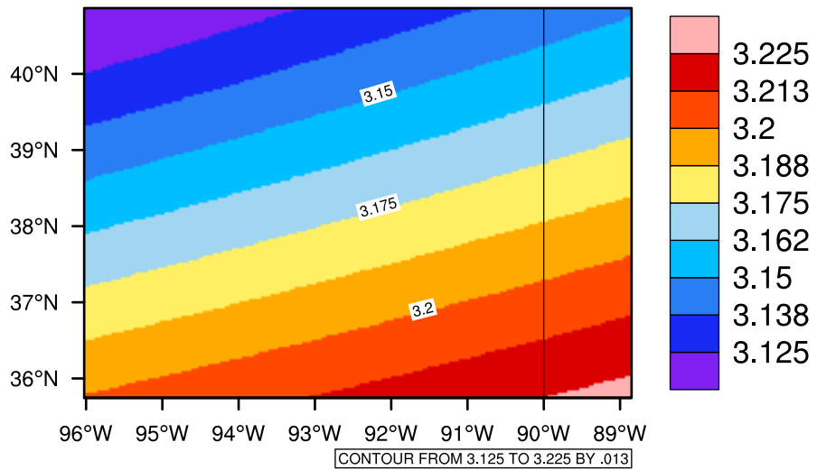
Yearly pr (mm/day) In 2050-2059 GFDL-ESM2M RCP45 - Missouri
