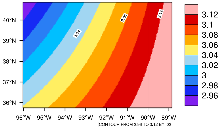
Yearly pr (mm/day) In 2070-2079 GFDL-ESM2M RCP45 - Missouri
