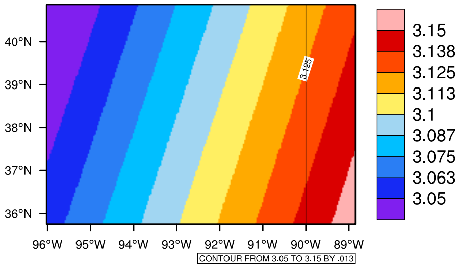
Yearly pr (mm/day) In 2080-2089 GFDL-ESM2M RCP45 - Missouri
