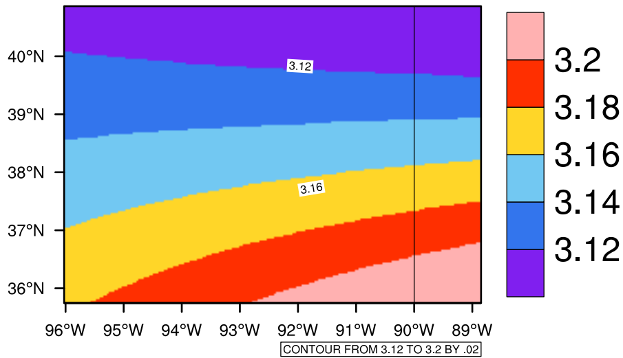
Yearly pr (mm/day) In 2020-2029 GFDL-ESM2M RCP85 - Missouri
