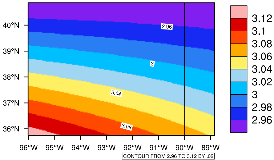
Yearly pr (mm/day) In 2030-2039 GFDL-ESM2M RCP85 - Missouri
