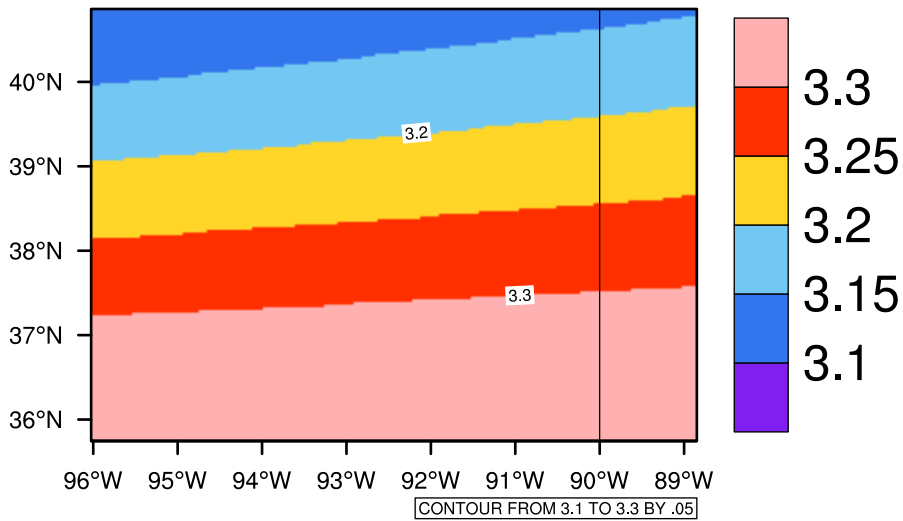
Yearly pr (mm/day) In 2040-2049 GFDL-ESM2M RCP85 - Missouri
