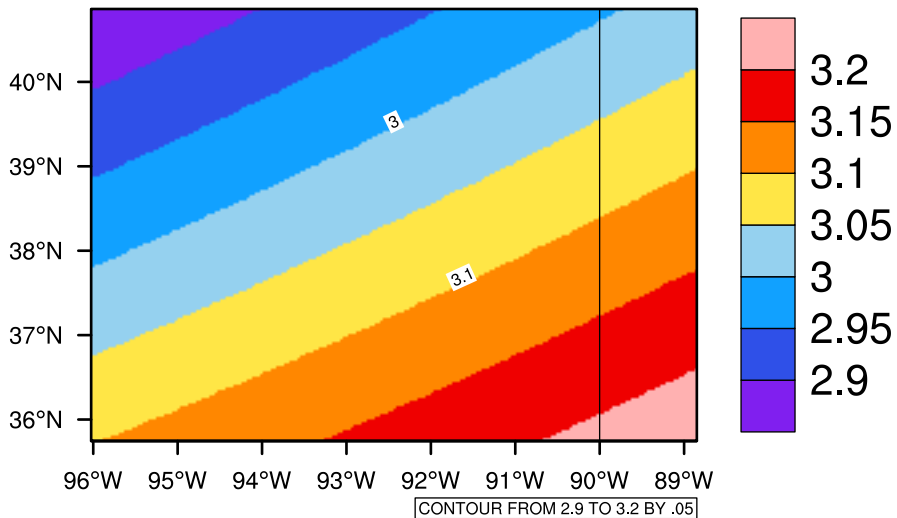
Yearly pr (mm/day) In 2050-2059 GFDL-ESM2M RCP85 - Missouri
