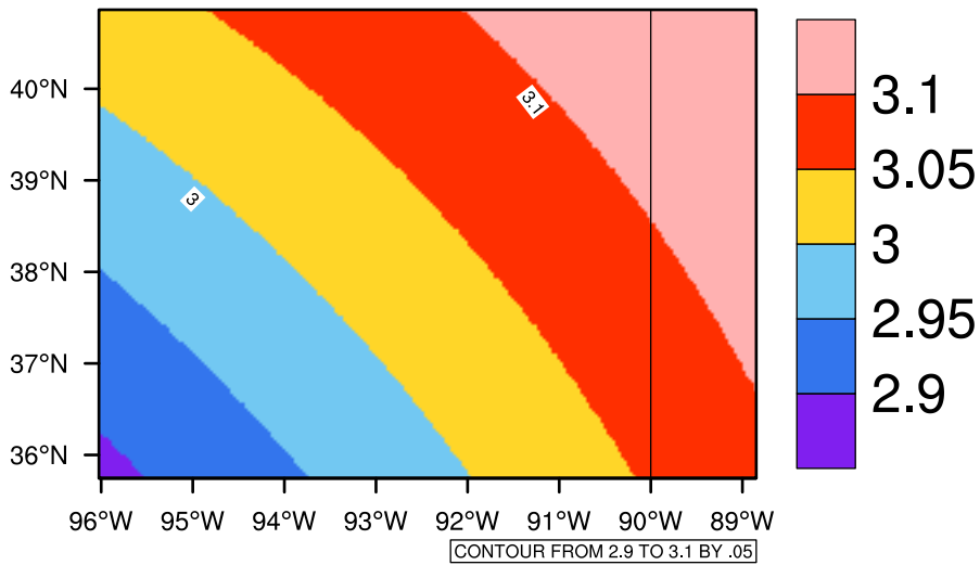
Yearly pr (mm/day) In 2060-2069 GFDL-ESM2M RCP85 - Missouri
