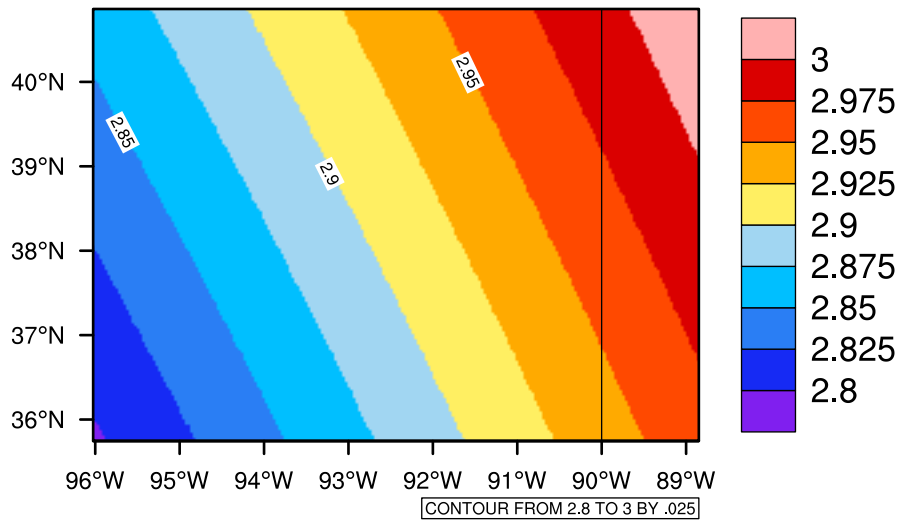
Yearly pr (mm/day) In 2070-2079 GFDL-ESM2M RCP85 - Missouri
