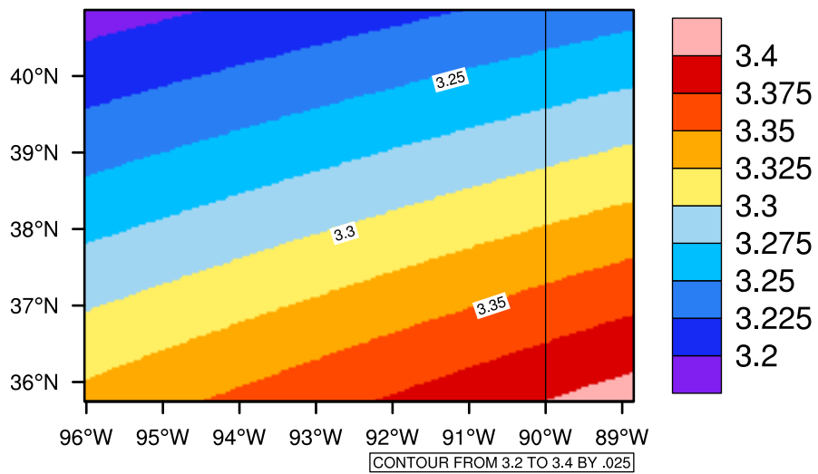
Yearly pr (mm/day) In 2080-2089 GFDL-ESM2M RCP85 - Missouri
