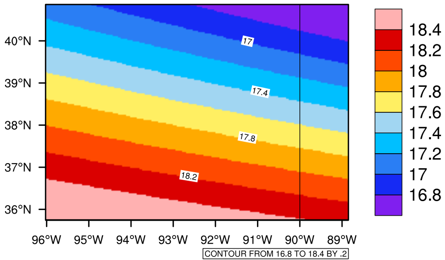
Yearly tasm max (c) In 2050-2059 GFDL-ESM2M RCP45 - Missouri
