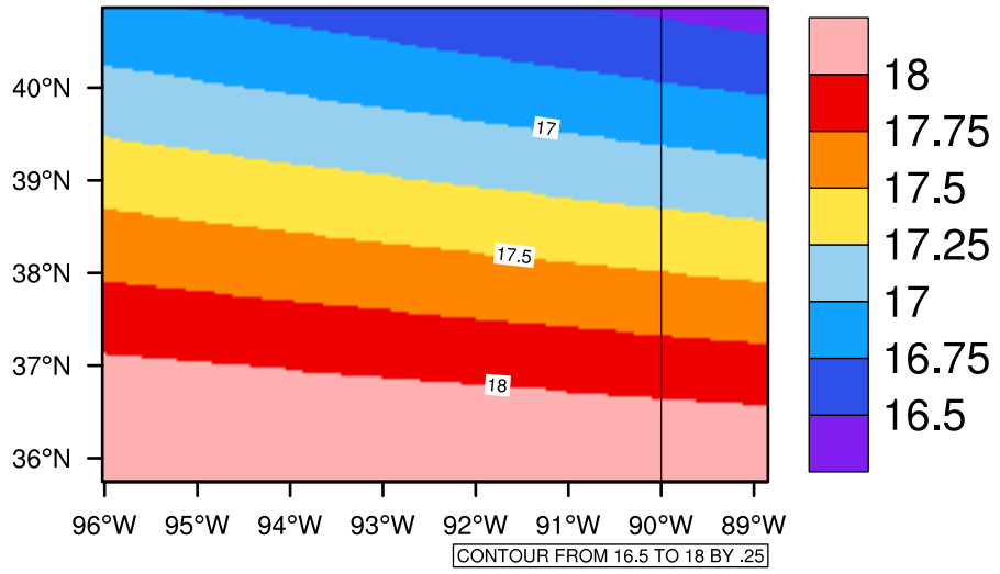
Yearly tasmax(c) In 2060-2069 GFDL-ESM2M RCP45 - Missouri
